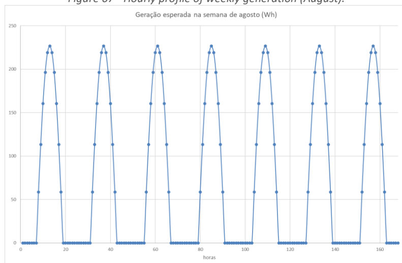
Figure 67 - Hourly profile of weekly generation (August).
