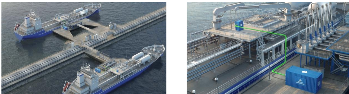
Figure 46 - Example of OPS installation for tankers: The Green Cable project for tankers at the Port of Gothenburg.
