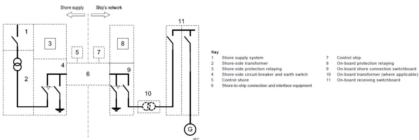
Figure 44 - General scheme of medium-voltage OPS connection.
