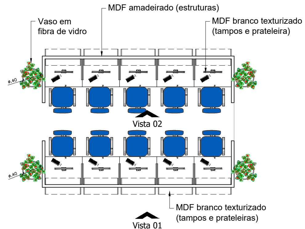
02 LAYOUT - MOB. MODULAR ESC: 1/50
